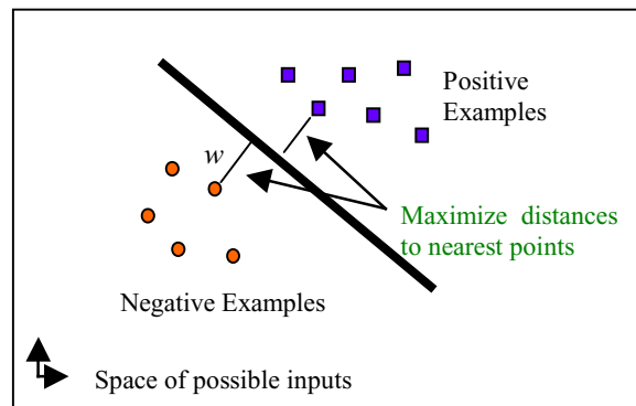
Figure 1 - Graphical Representation of a Linear SVM
